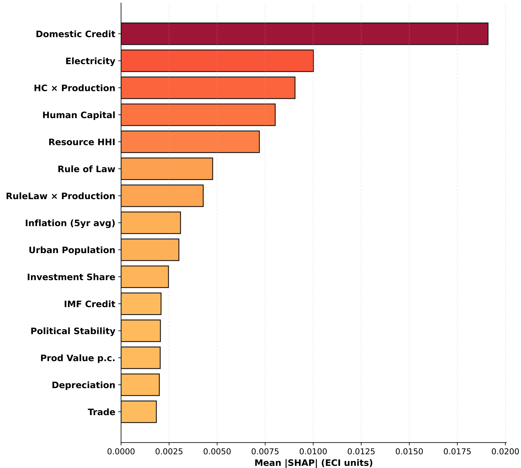
SHAP — Random Forest (test set)
