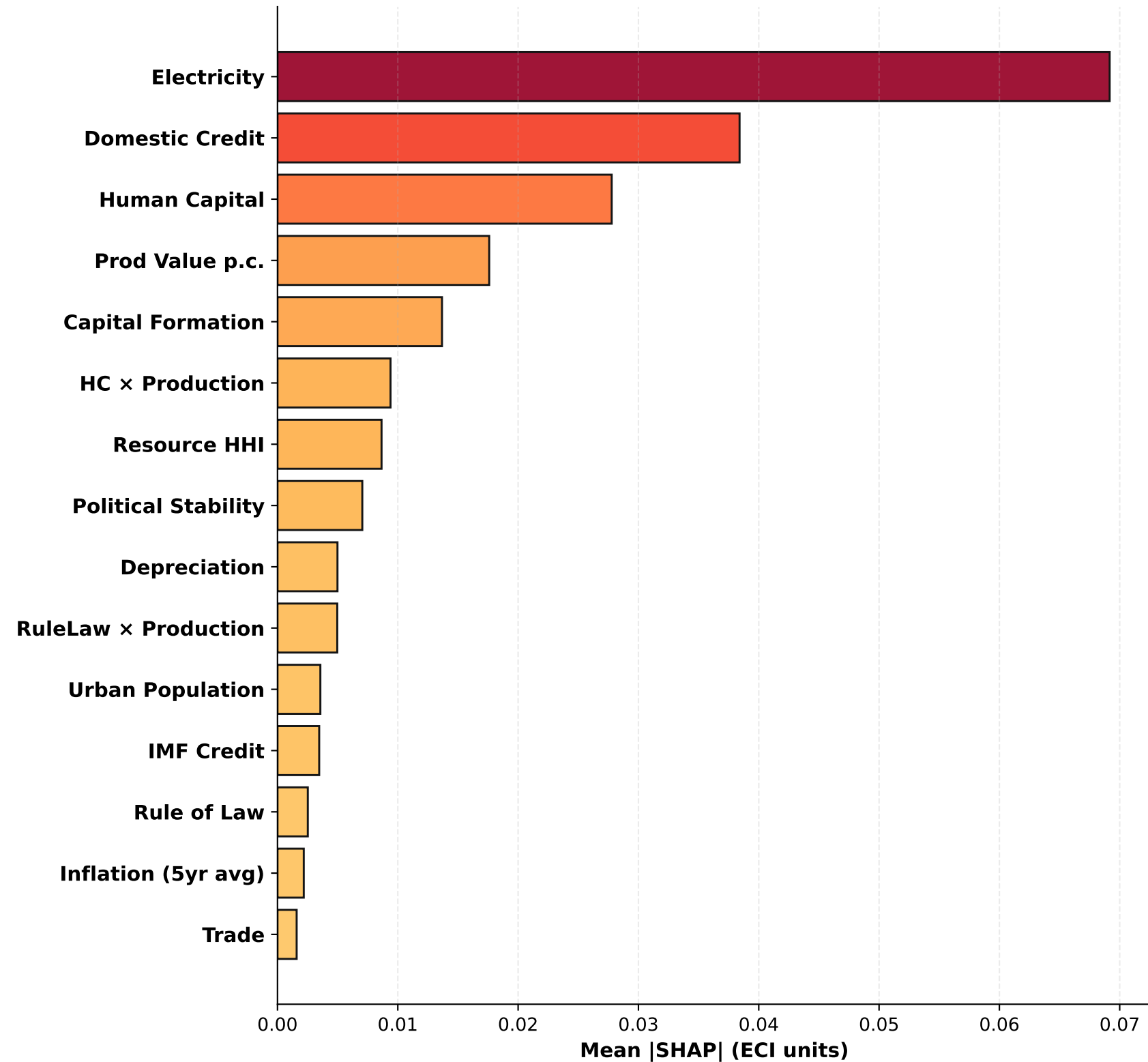
SHAP — XGBoost (test set)
